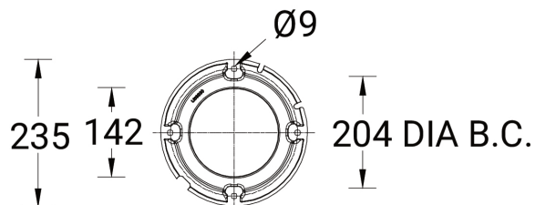
Mounting detail
