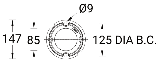
Mounting detail
